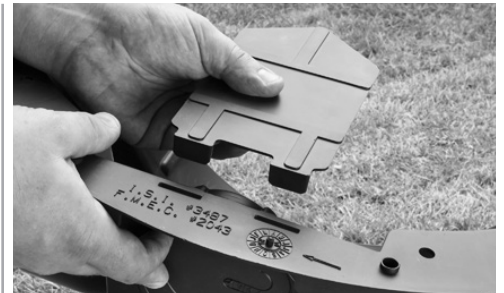
4. Install splash plate.
